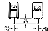
08 Printed Circuit
