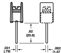
07 Extended Pin
